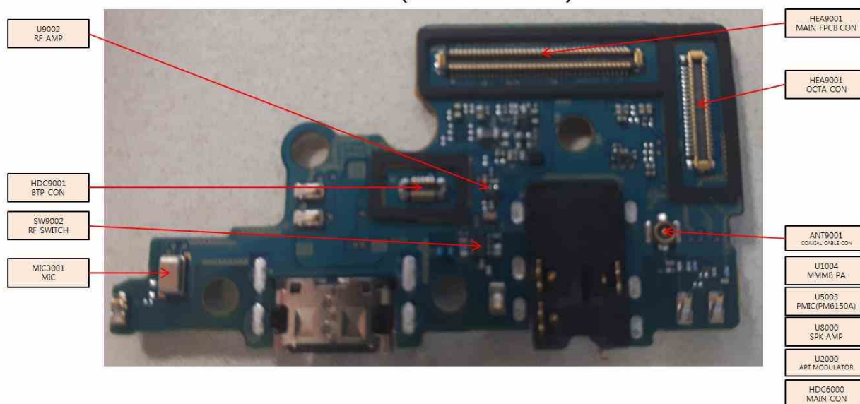
SUB PBA (BOTTOM SIDE)
